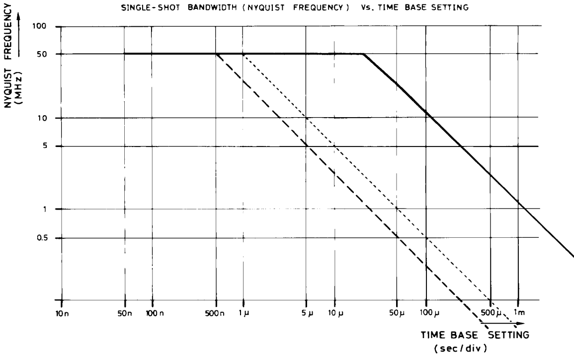
Single-shot bandwidth is a function of sampling rate. Long memories enable higher sampling rates at equal time-base settings. Above, the 9400A (solid line) is compared to oscilloscopes with 1K (dotted line) and 512 points (dashed line) of memory. At slower time-base settings, the single-shot bandwidth of the 9400A, expressed as Nyquist frequency, is typically 25 times higher than in oscilloscopes with 1K memory and 50 times higher than in those with only 512 points.
